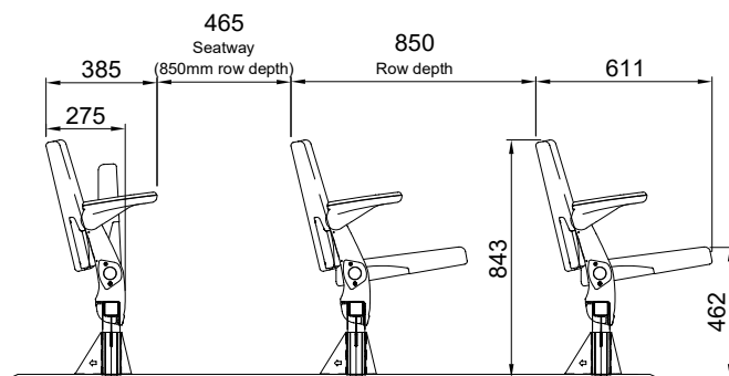
SIDE VIEW ON SEATING
