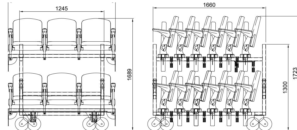
FRONT VIEW ON SEATING STORAGE
