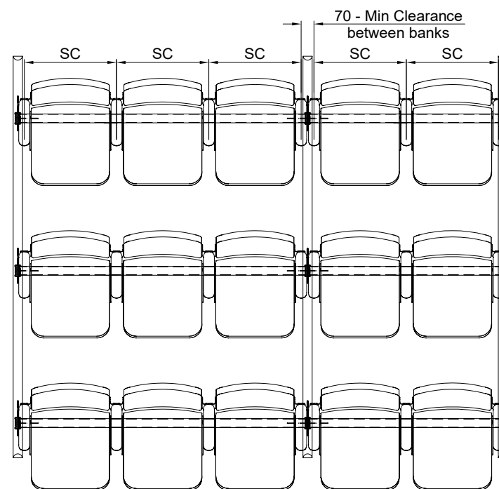
PLAN VIEW ON SEATING
