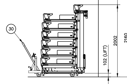
ELEVATION ON LIFTED SEATING UNIT (SIDE RAILS NOT SHOWN FOR CLARITY)
