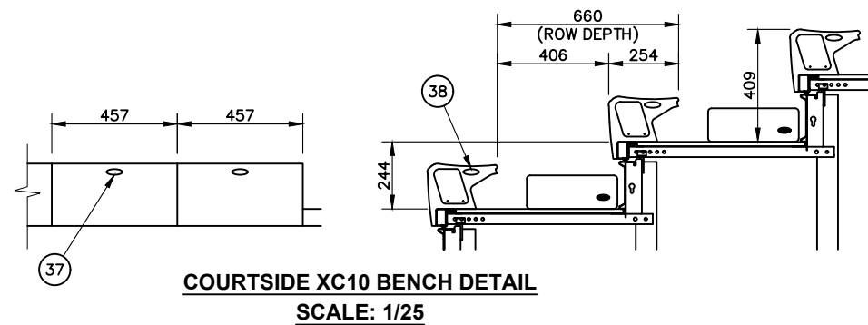
BANKS A1, A4 & B TYPICAL
