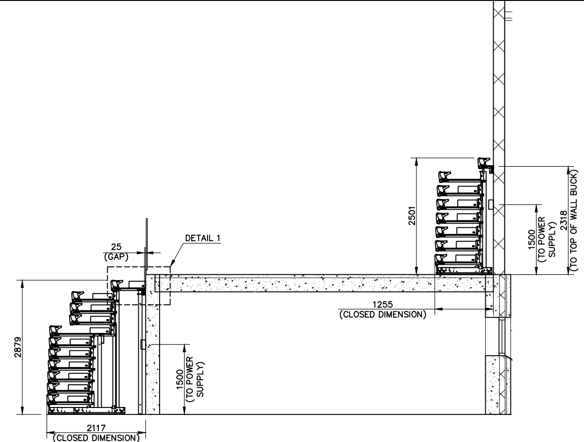
ELEVATION ON CLOSED SEATING UNIT (SIDE RAILS NOT SHOWN FOR CLARITY)
