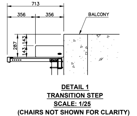
BANKS A12, A22, A33 & A44 TYPICAL (WALL ATTACHED)
