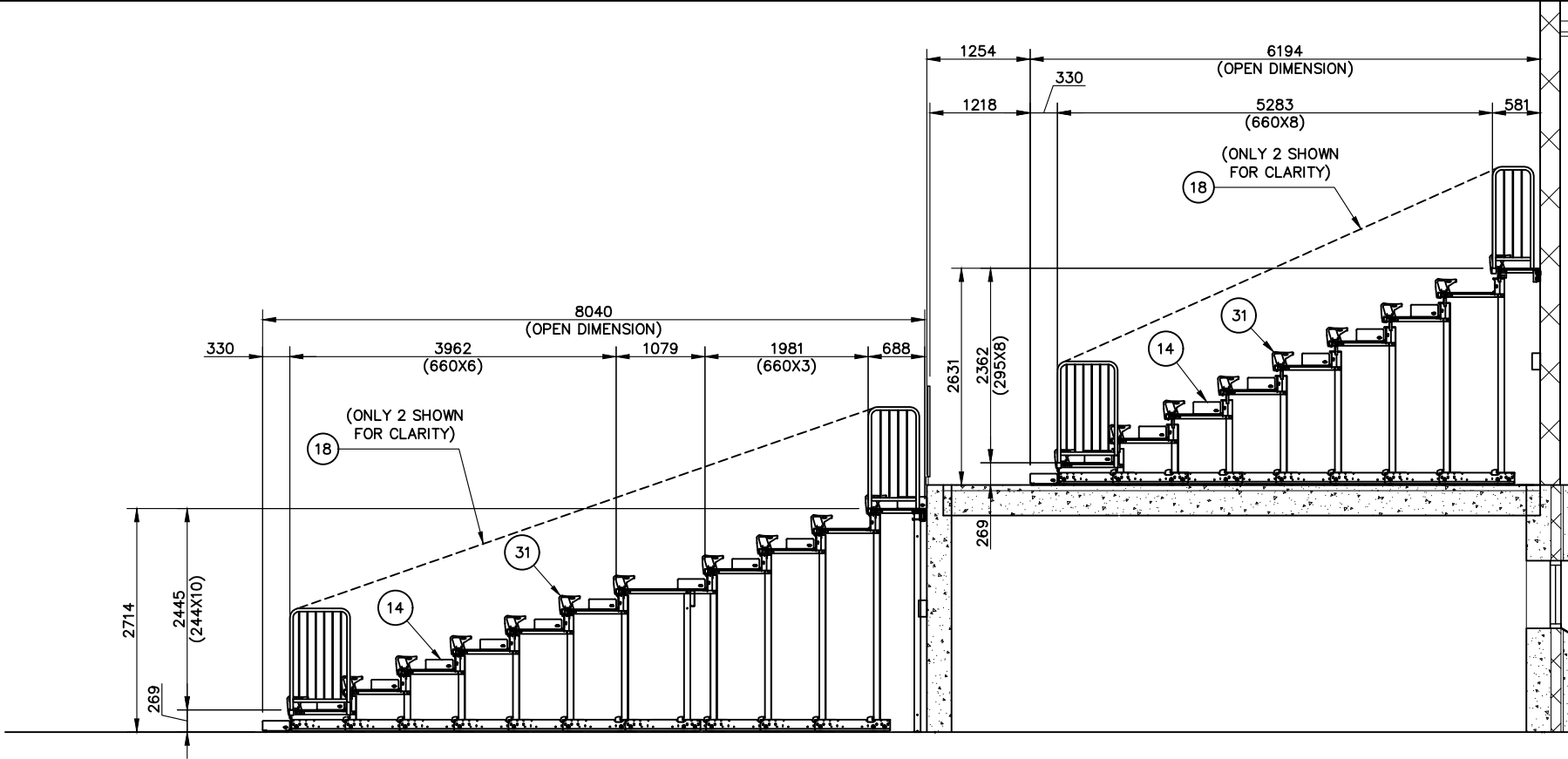
ELEVATION ON EXTENDED SEATING UNIT
