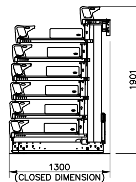
ELEVATION ON CLOSED SEATING UNIT (SIDE RAILS NOT SHOWN FOR CLARITY)
