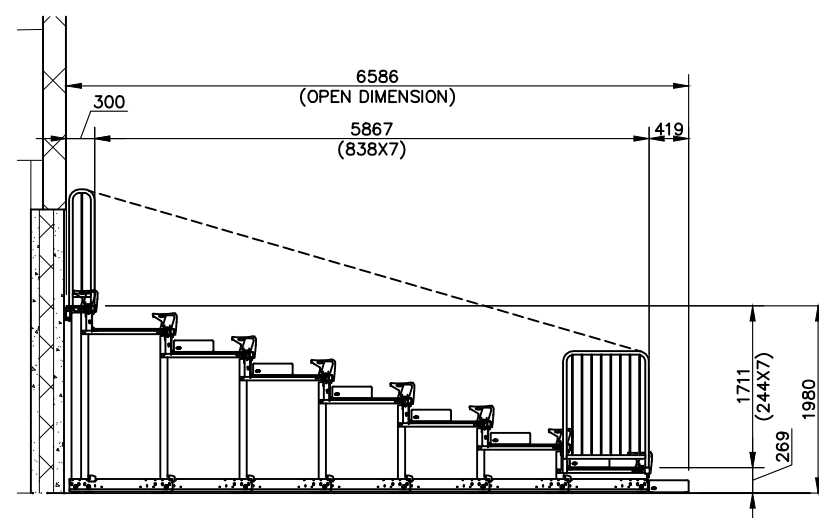
ELEVATION ON EXTENDED SEATING UNIT
