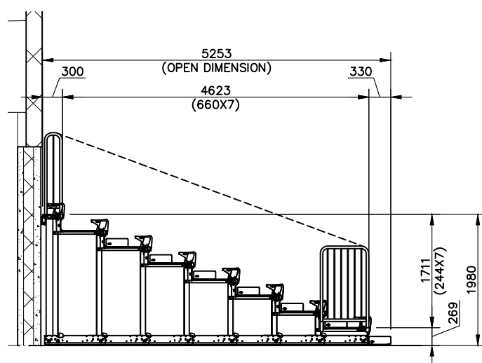
ELEVATION ON EXTENDED SEATING UNIT
