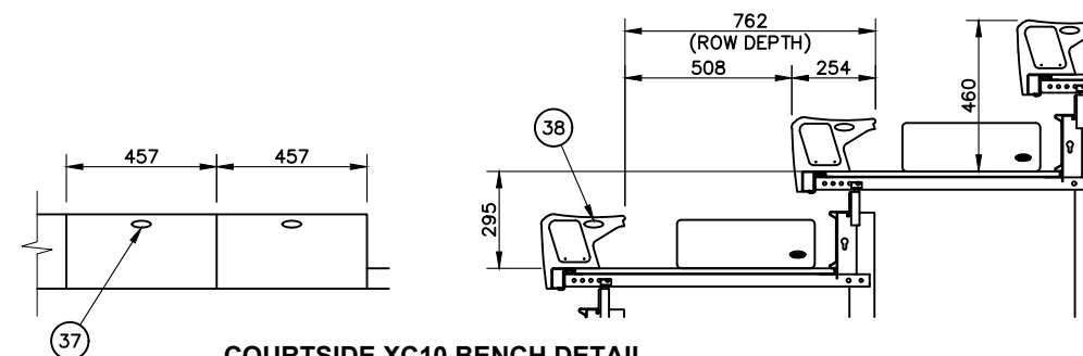
COURTSIDE XC10 BENCH DETAIL SCALE: 1/25
