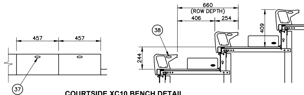
COURTSIDE XC10 BENCH DETAIL SCALE: 1/25
