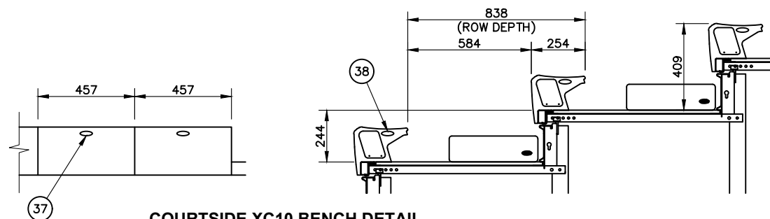
COURTSIDE XC10 BENCH DETAIL SCALE: 1/25
