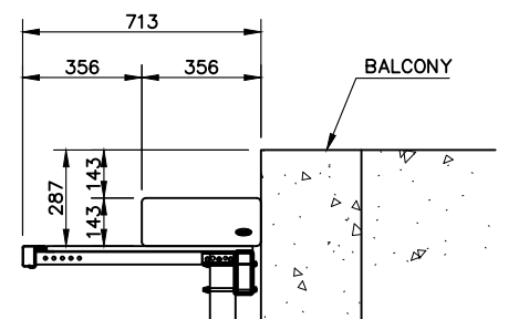
DETAIL 2 TRANSITION STEP SCALE: 1/25 (CHAIRS NOT SHOWN FOR CLARITY)
