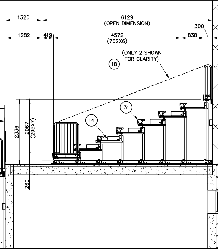
ELEVATION ON EXTENDED SEATING UNIT
