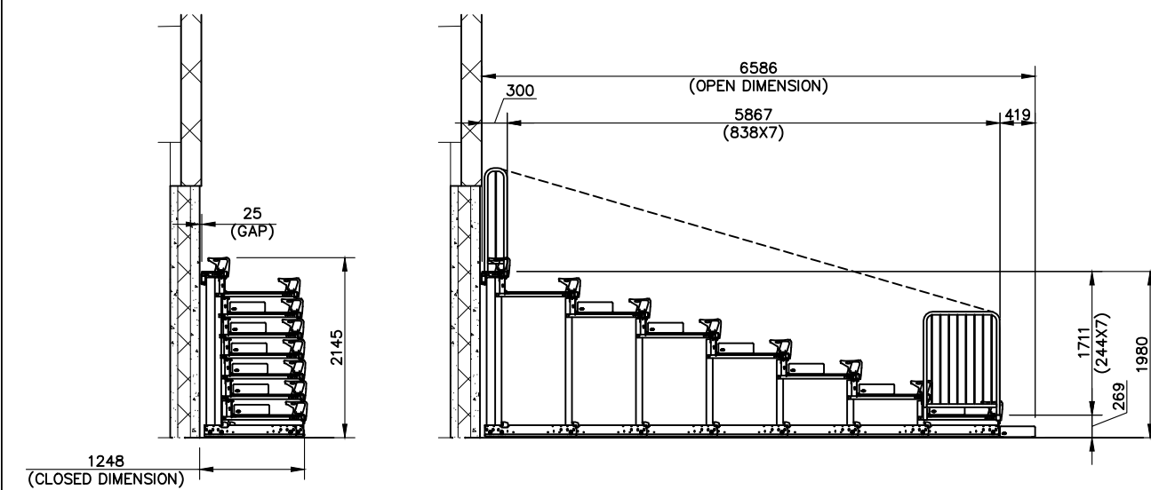
ELEVATION ON CLOSED SEATING UNIT (SIDE RAILS NOT SHOWN FOR CLARITY)
