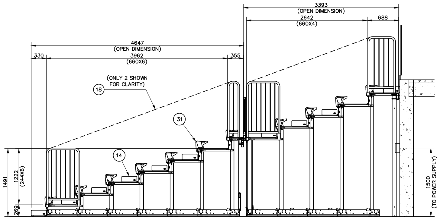
ELEVATION ON EXTENDED SEATING UNIT
