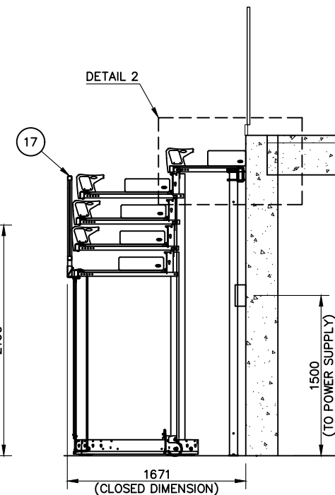
ELEVATION ON CLOSED SEATING UNIT (SIDE RAILS NOT SHOWN FOR CLARITY)
