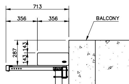
DETAIL 2 TRANSITION STEP SCALE: 1/25 (CHAIRS NOT SHOWN FOR CLARITY)
