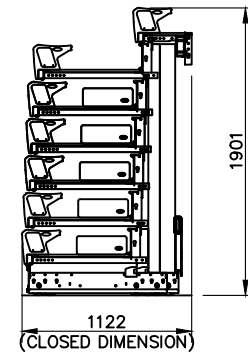
ELEVATION ON CLOSED SEATING UNIT (SIDE RAILS NOT SHOWN FOR CLARITY)
