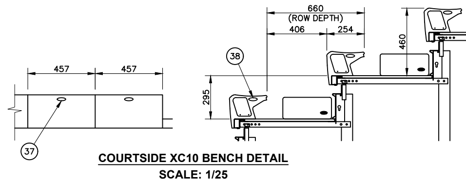
BANKS A12, A22, A33 & A44 TYPICAL
