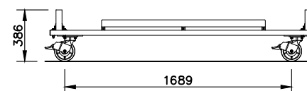
TRANSPORTABLE RAIL TROLLEY DETAIL (42 PCS PER TROLLEY) SCALE: 1/40
