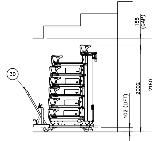
ELEVATION ON LIFTED SEATING UNIT (SIDE RAILS NOT SHOWN FOR CLARITY)
