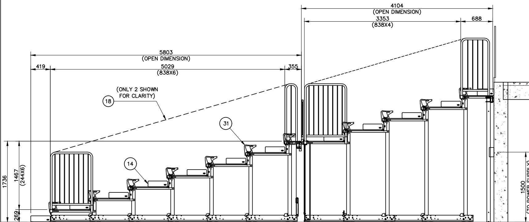
ELEVATION ON EXTENDED SEATING UNIT
