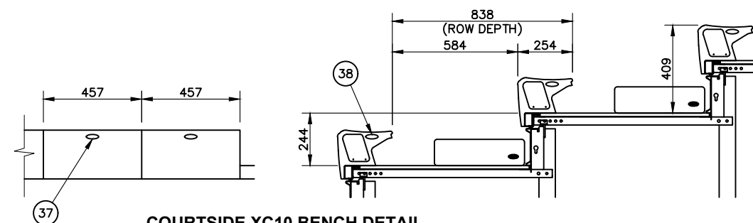
COURTSIDE XC10 BENCH DETAIL SCALE: 1/25
