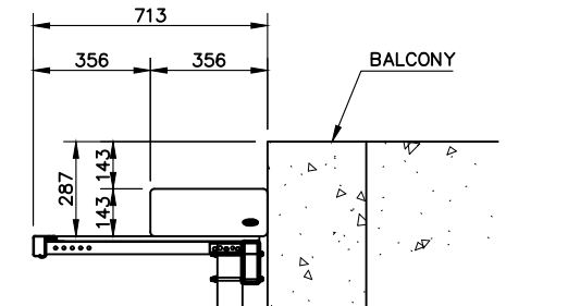
DETAIL 1 TRANSITION STEP SCALE: 1/25 (CHAIRS NOT SHOWN FOR CLARITY)
