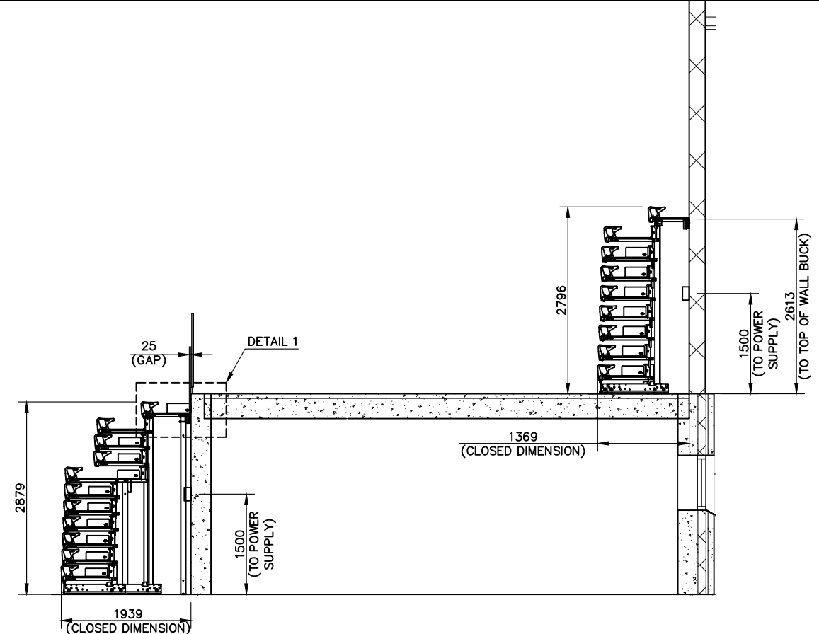
ELEVATION ON CLOSED SEATING UNIT (SIDE RAILS NOT SHOWN FOR CLARITY)
