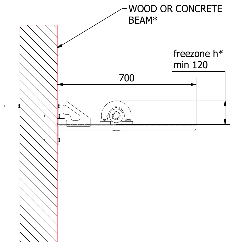
SECTION C-C
