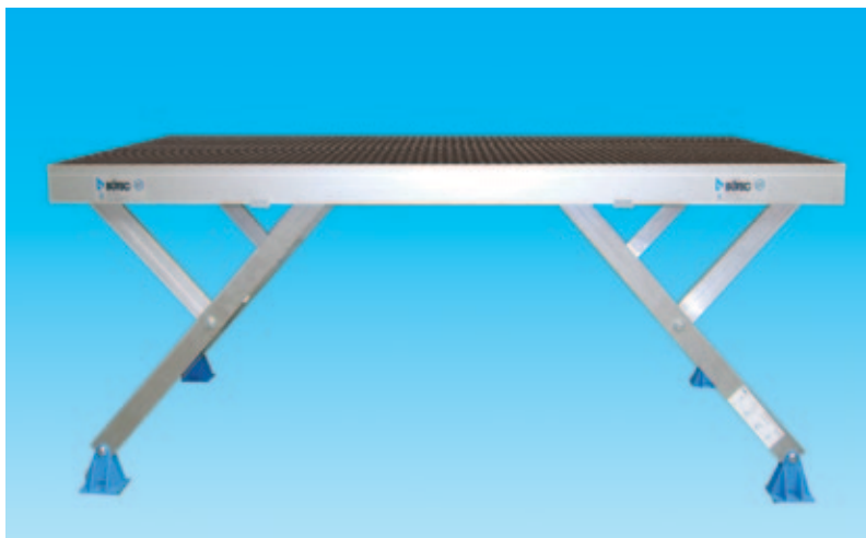
Scissor platform BÜTEC 100 here with screen print plate for outdoor use – water-proof laminated multi-layer plate, colour: dark Swivel feet with large contact areas provide a good load distribution, and a hinge allows compensation for sloping floors – without wobbling
