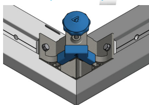
Leg Attachment Corner (welded)
