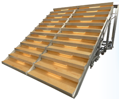
Stairs made to Measure, rollable on request
